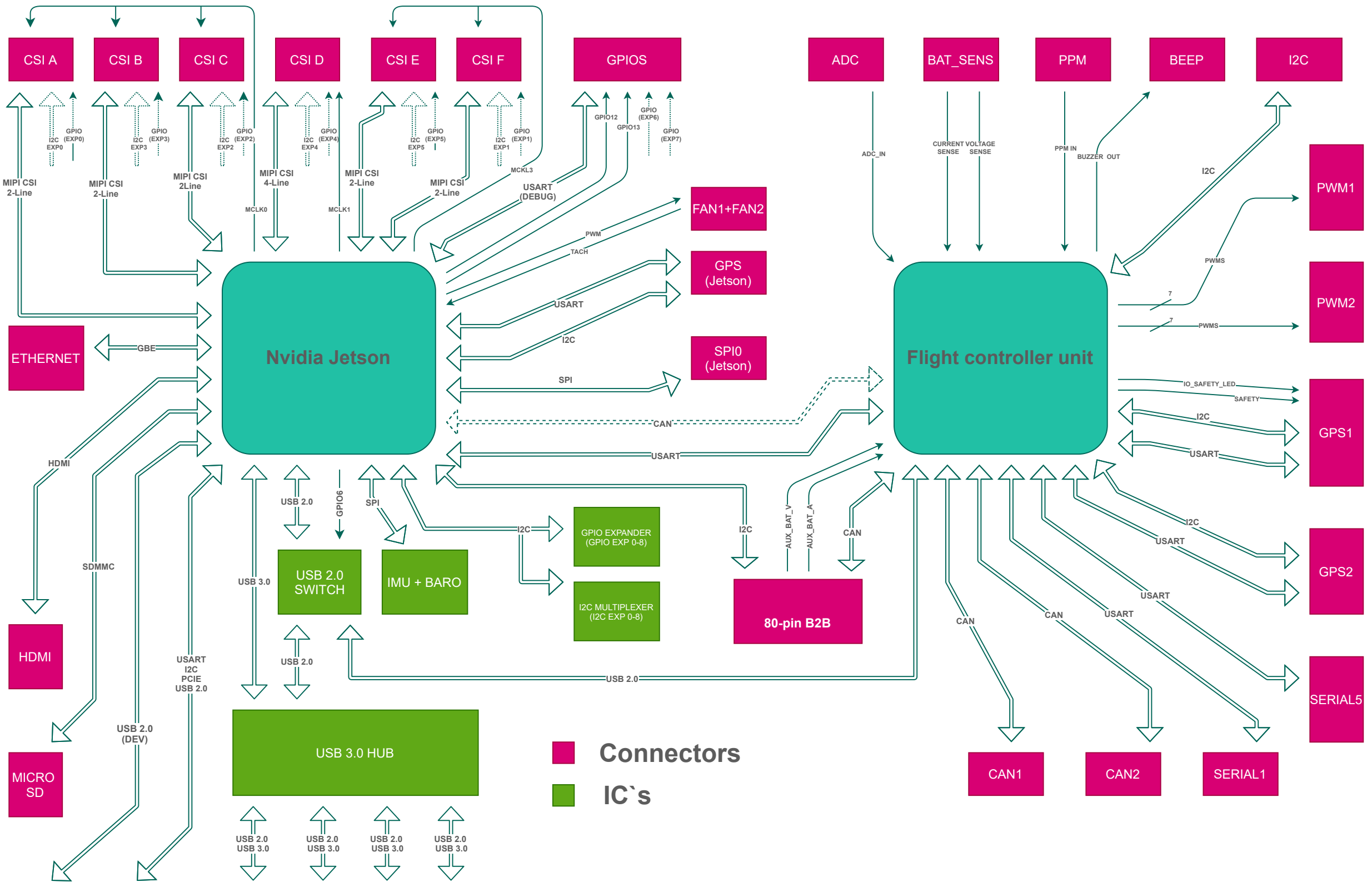
DroneCore.Pilot peripherals block diagram
